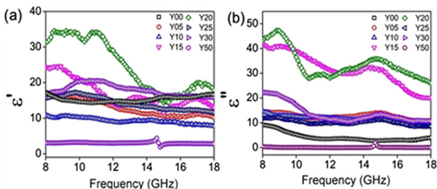
Figure 9. (a) \epsilon' and (b) \epsilon'' as a function of YIG content in PANI/YIG composite in the frequency range between 8 and 18 GHz. Reproduced with permission from ref. 104 Copyrights © 2011 2018 Wiley-VCH Verlag GmbH & Co. KGaA, Weinheim.
