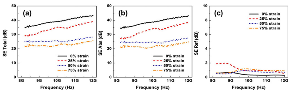
Figure 29. SET, (b) SEA, (c) SER of the 6 mm thick G (10 wt.%) / PU under various compression strain in the frequency range of 8–12 GHz. Modified from ref. 236
